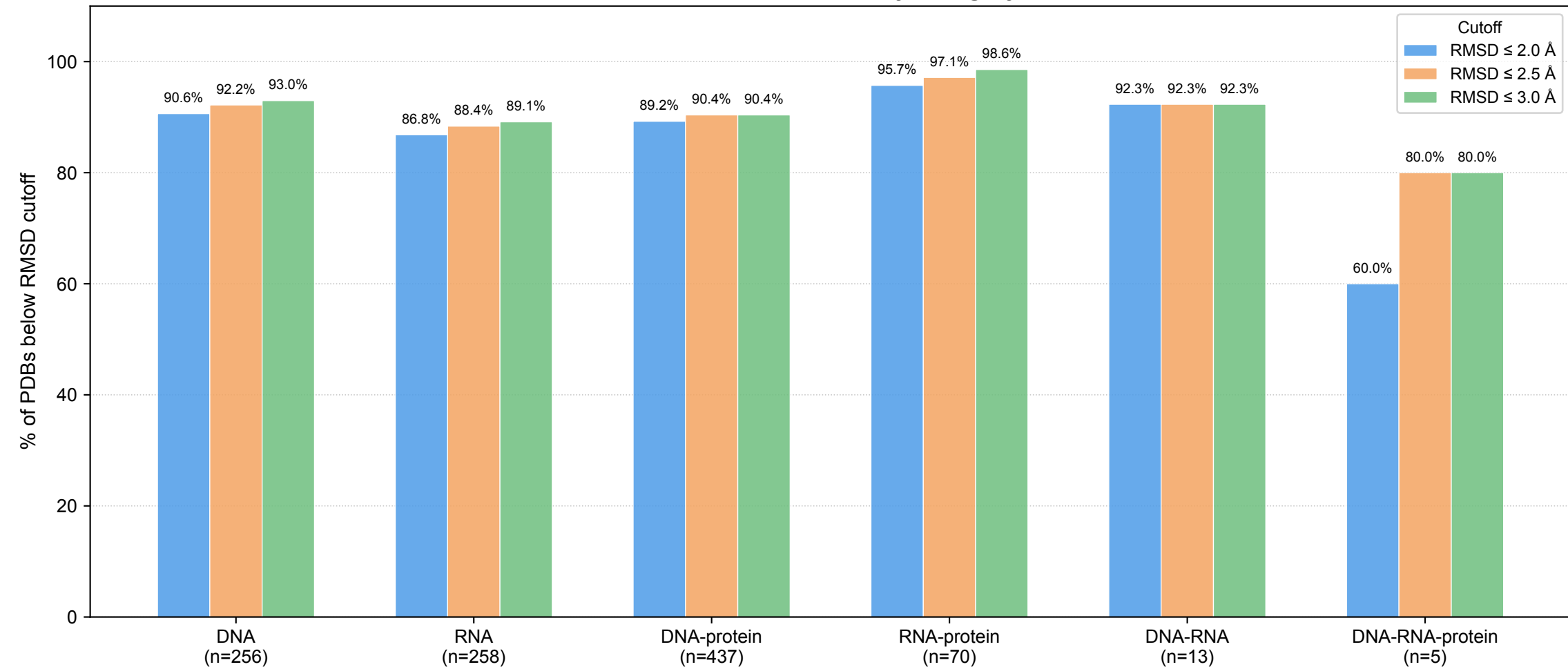
Full Structure RMSD by Category
