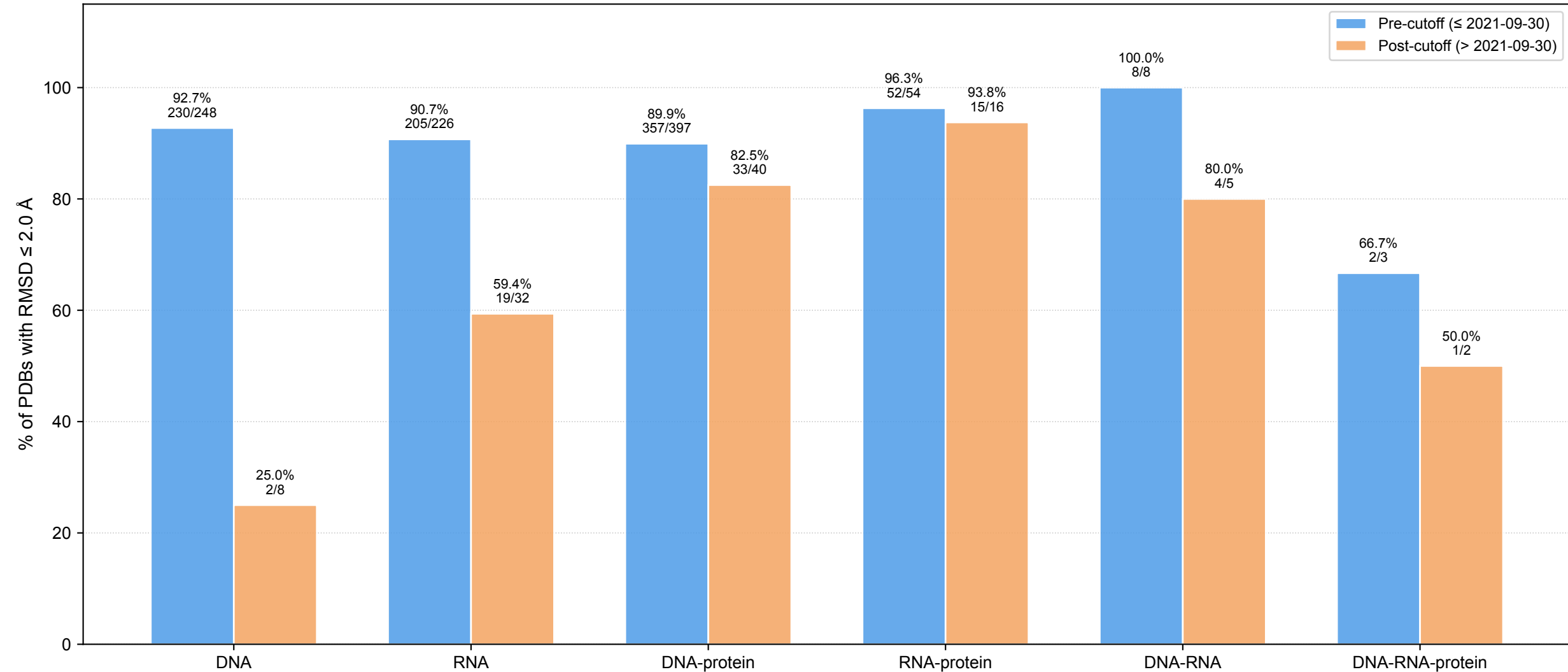
Full Structure RMSD \leq 2.0 Å by Category and Release Period
