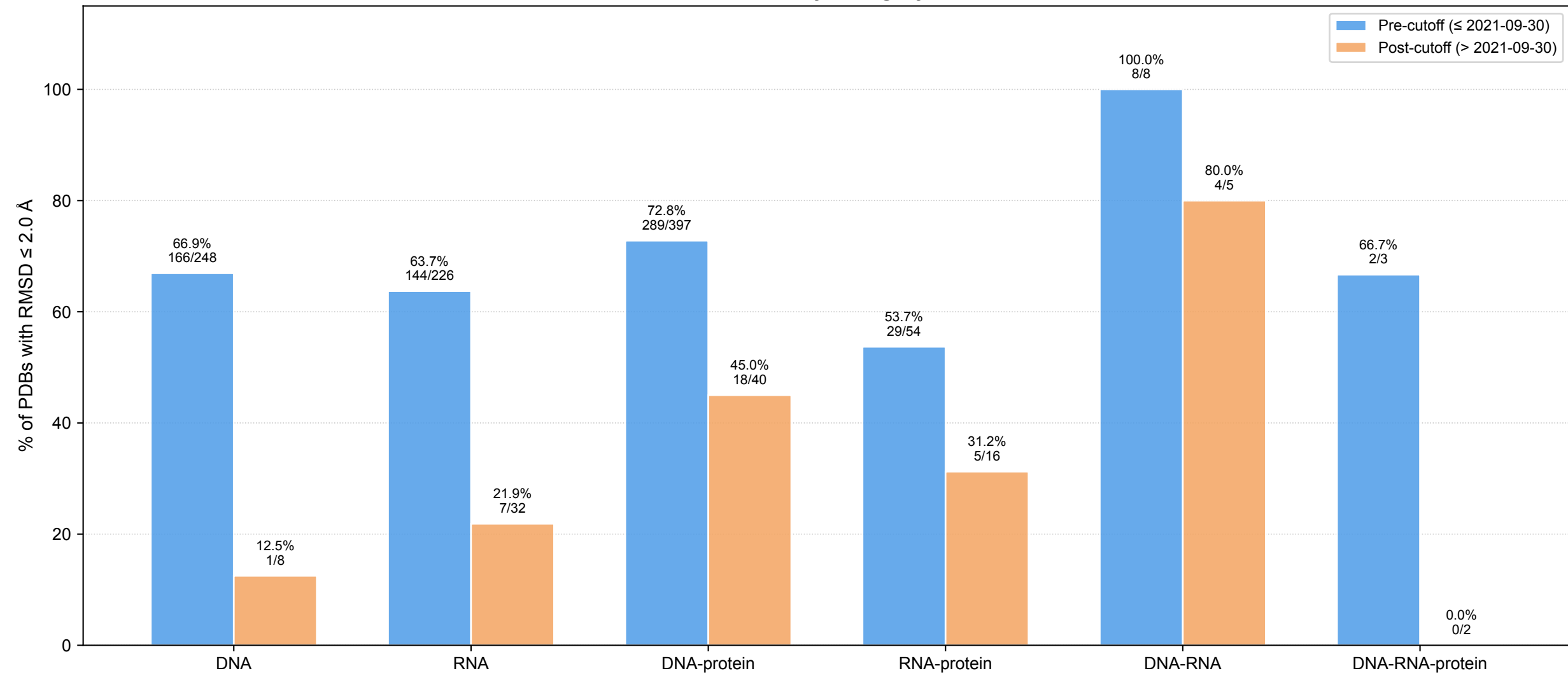
Modification RMSD \leq 2.0 Å by Category and Release Period
