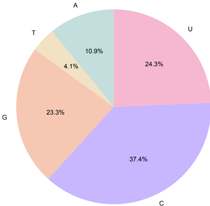
Distribution of Modified Bases (A,T,G,C,U) — per-PDB presence
