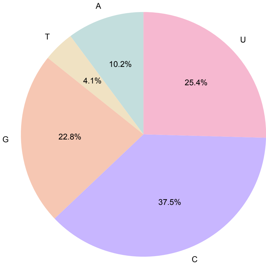
Distribution of Modified Bases – PRE
