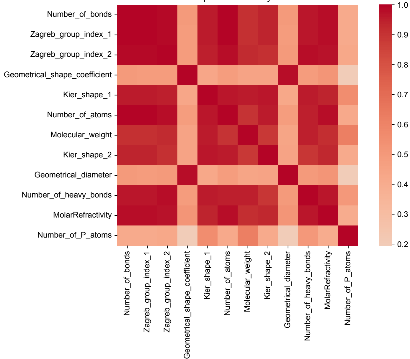
C. Descriptor redundancy structure
