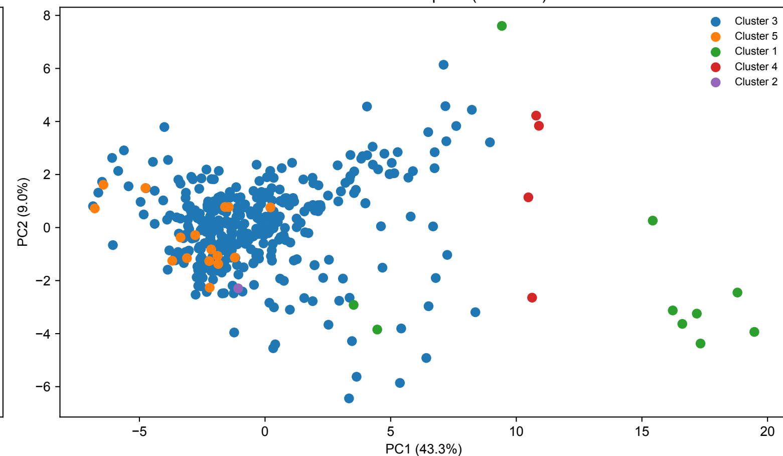
B. PCA chemical space (clustered)
