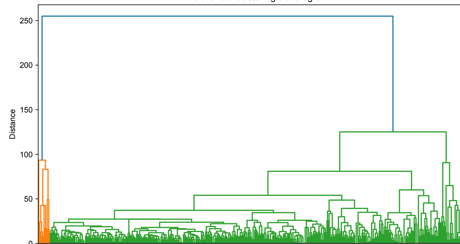
D. Hierarchical clustering dendrogram
