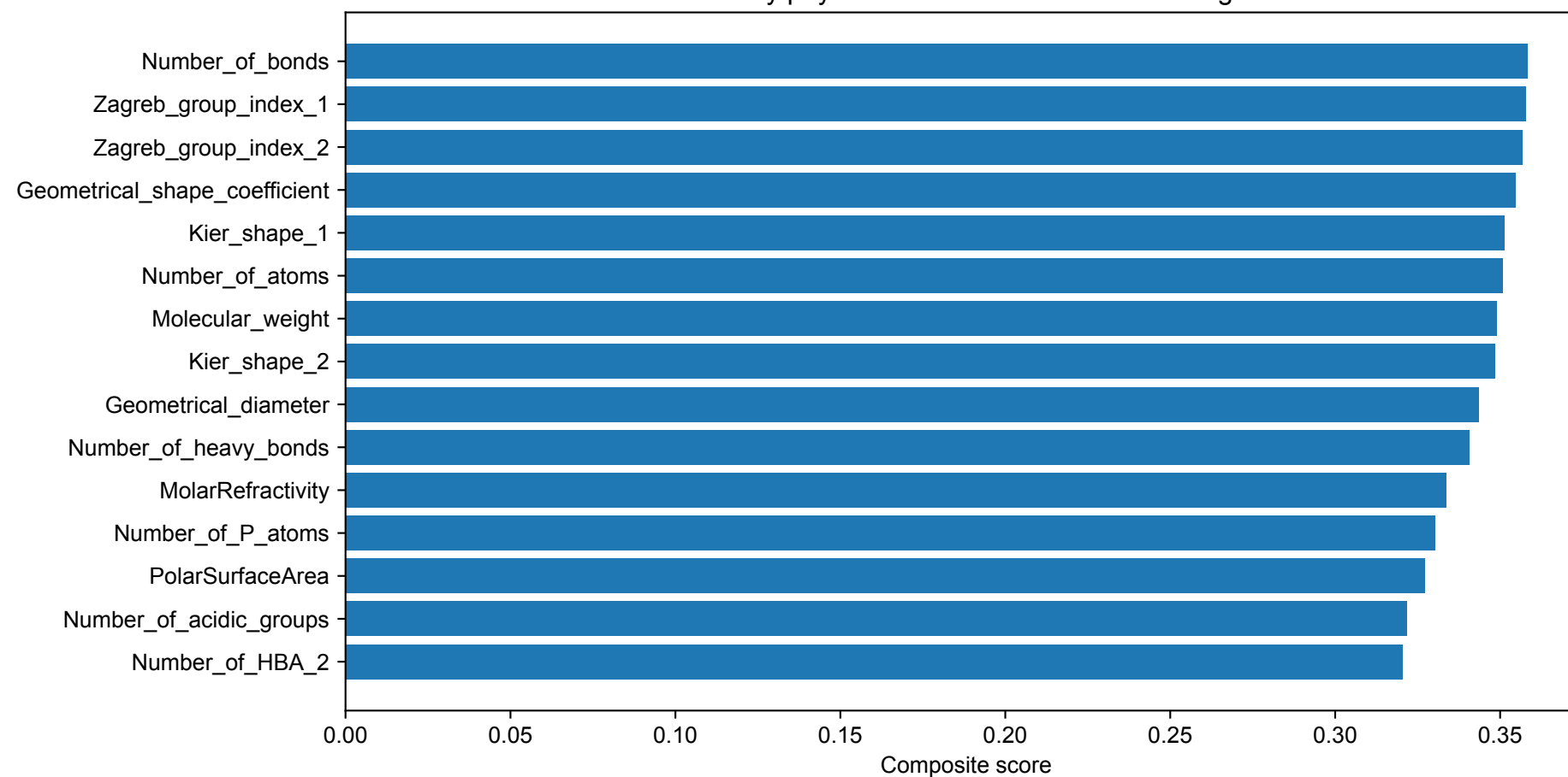
A. Key physicochemical drivers of clustering
