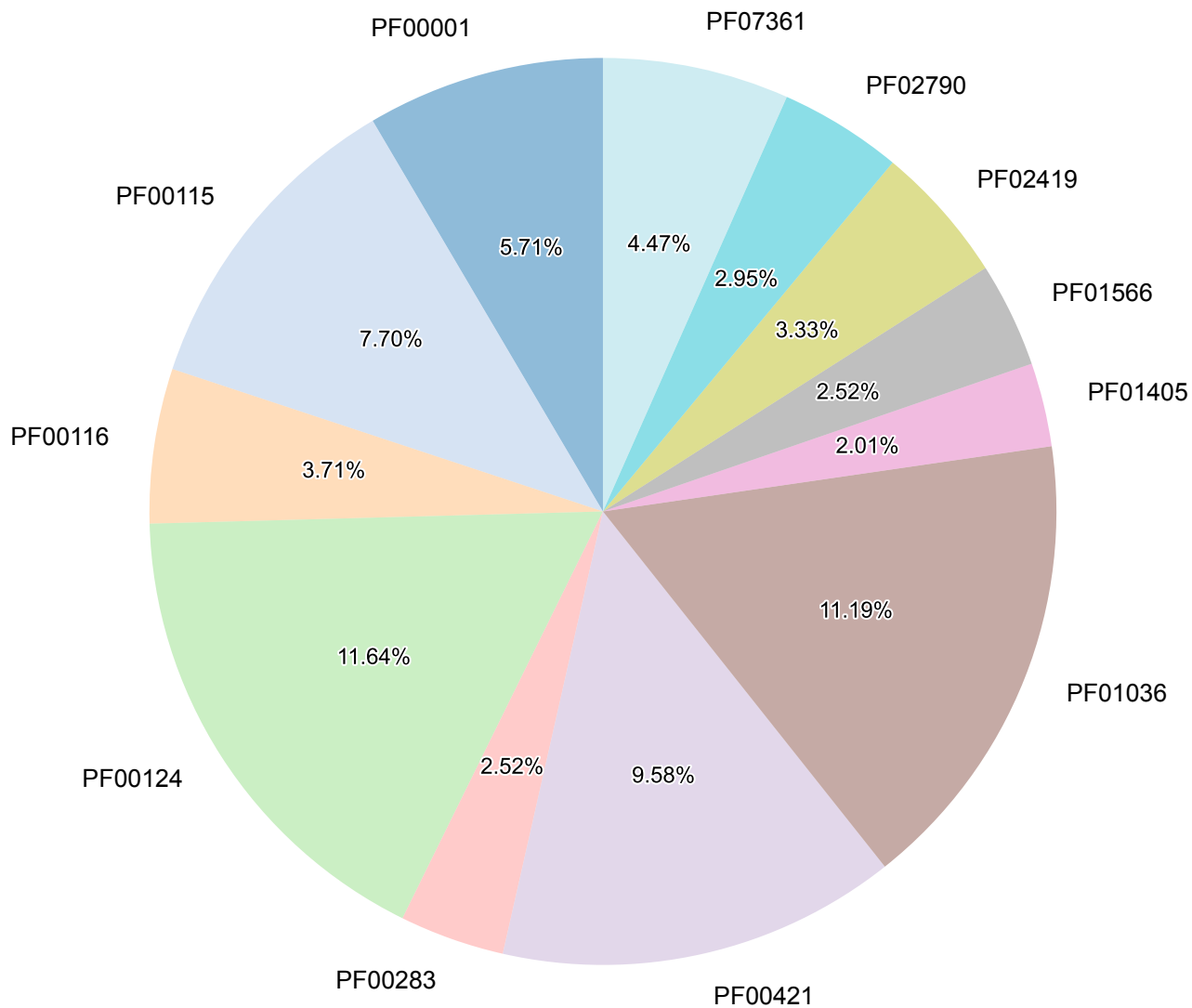
PFAM distribution (>1% frequency)
