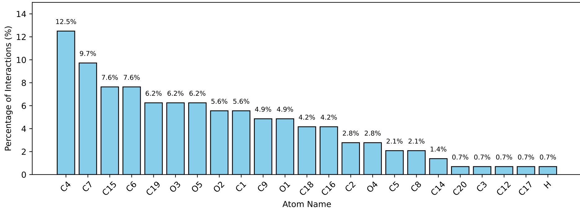
Percentage of Interactions per HCY Atom
