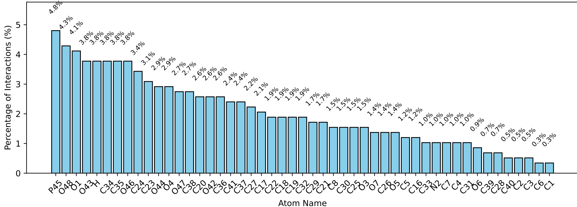
Percentage of Interactions per LP5 Atom
