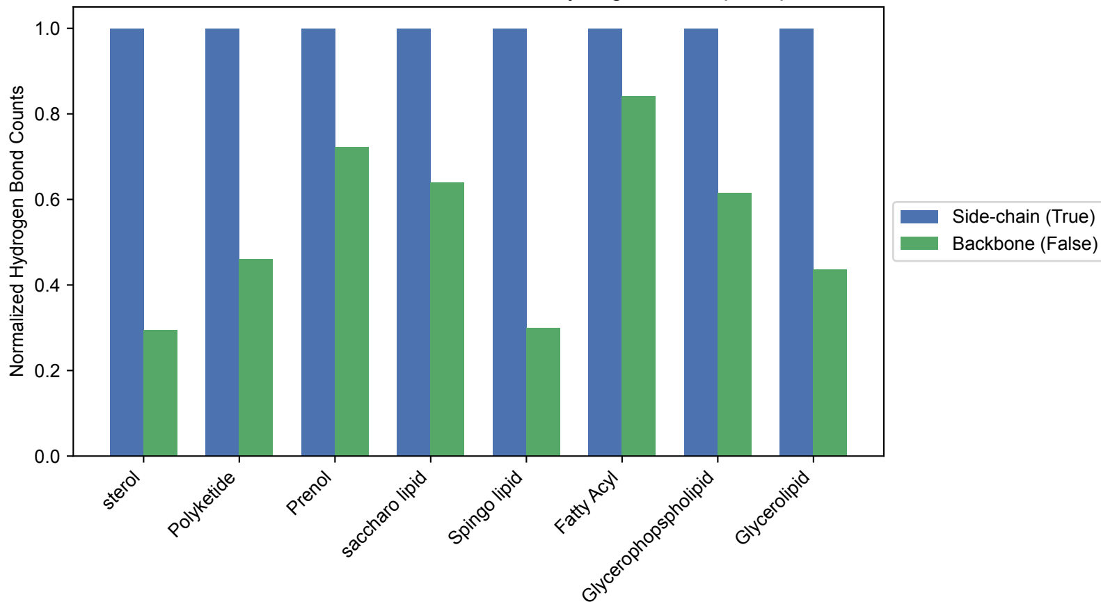
Normalized Counts of Side-chain vs Backbone Hydrogen Bonds per Lipid Class
