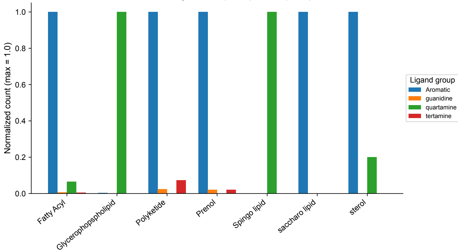
Normalized \pi -cation Ligand Group Frequencies per Lipid Class
