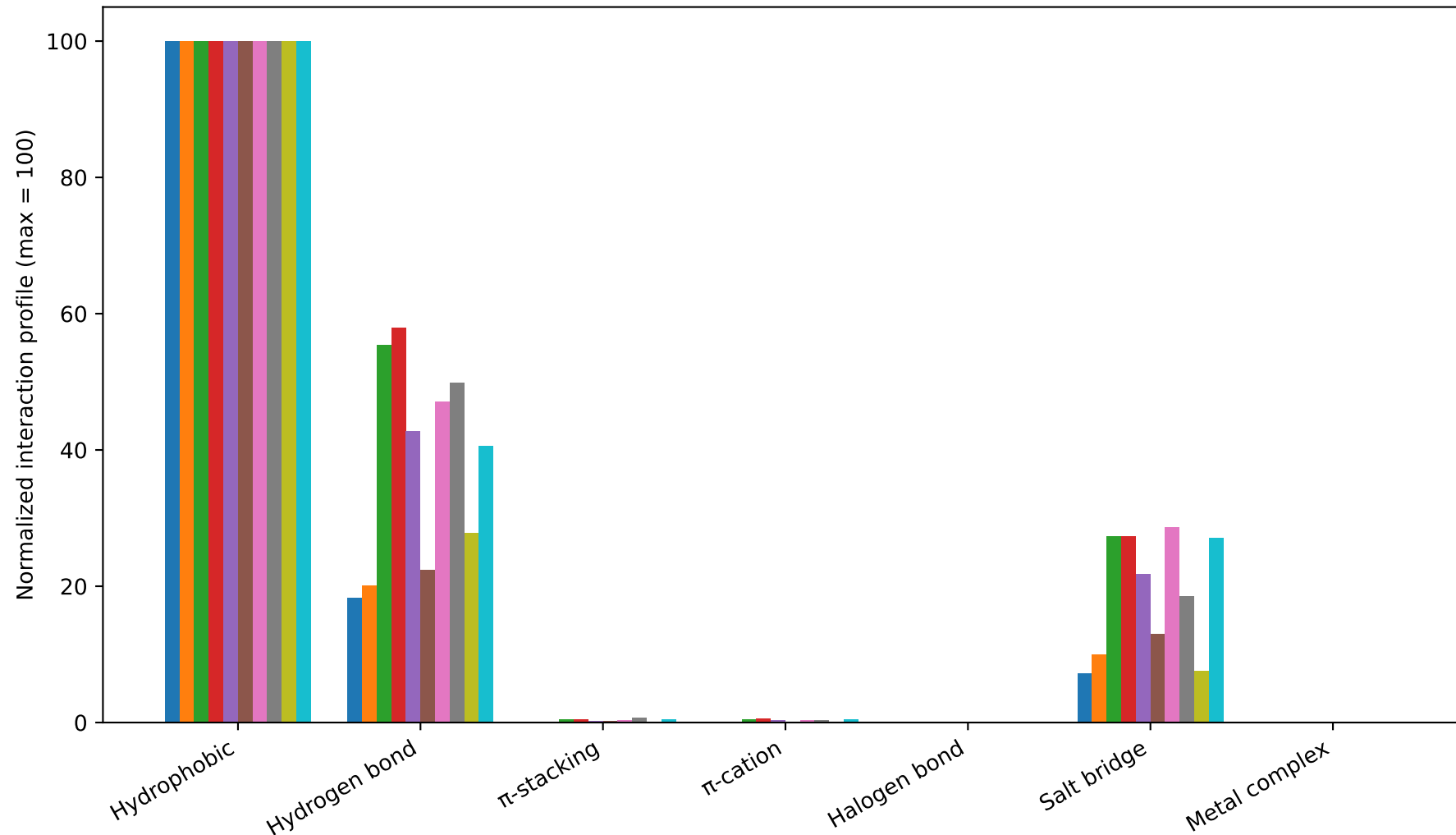
fattyacyls-Protein Interaction Profiles by Subcellular Location
