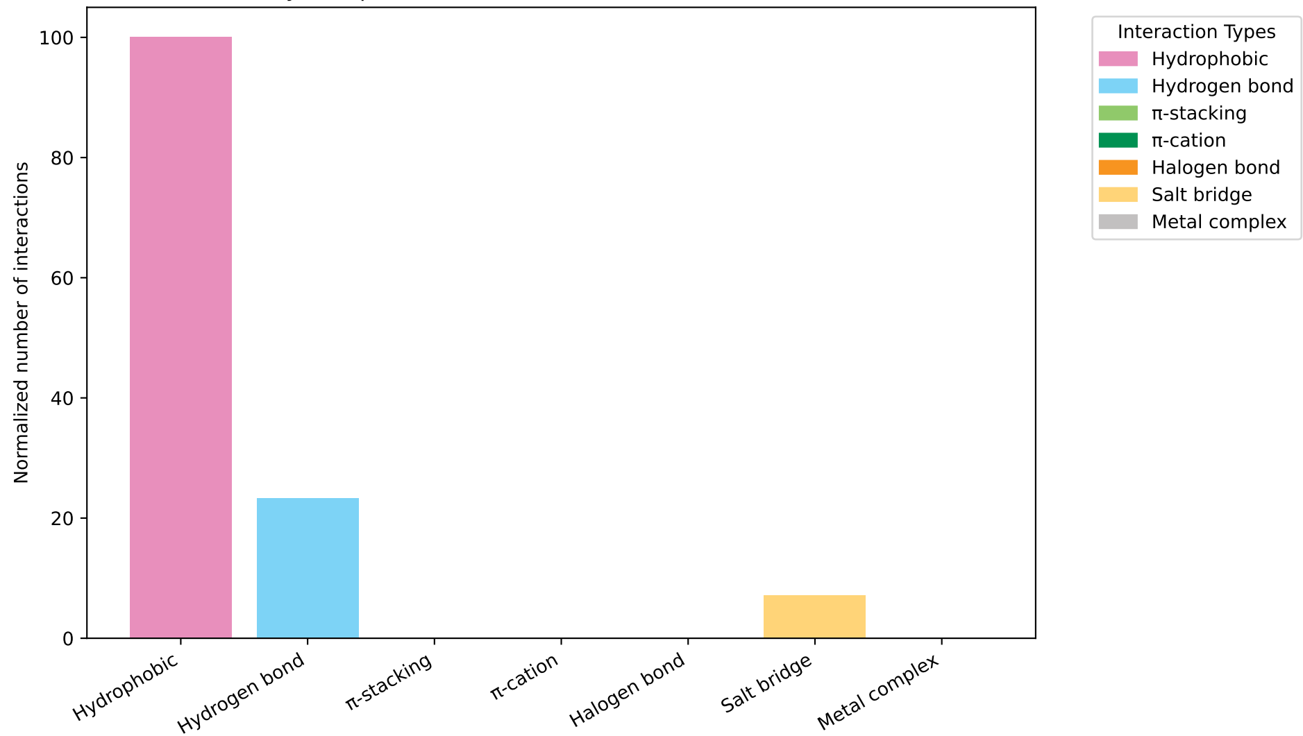
Glycerolipids-Protein Interaction Profiles (Normalized)
