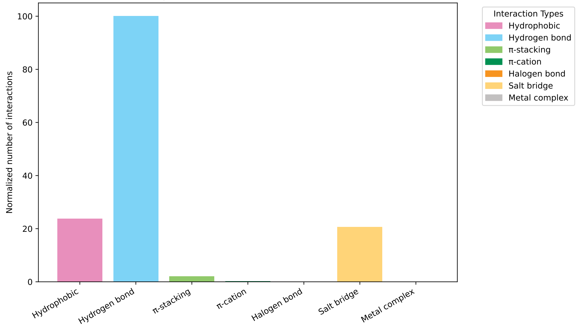
Saccharolipids-Protein Interaction Profiles (Normalized)
