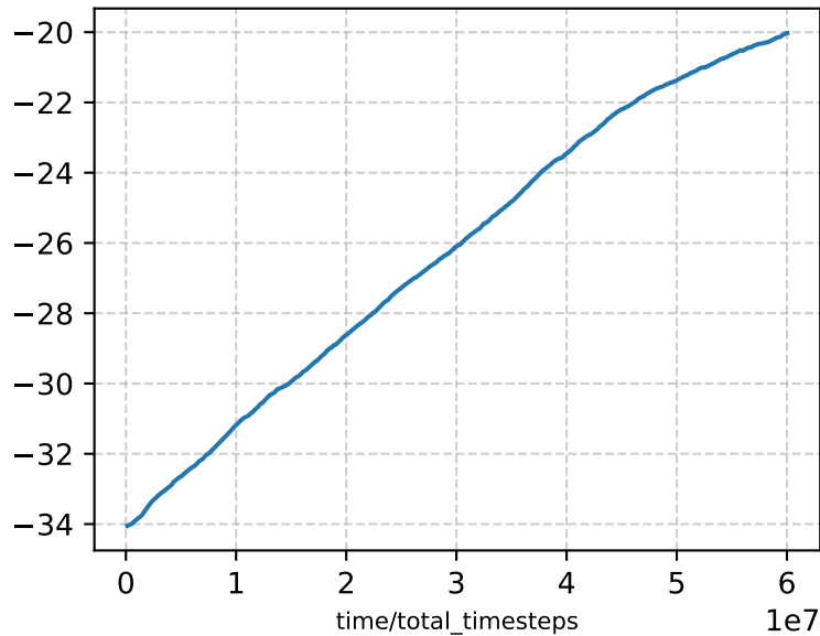
train/entropy_loss
