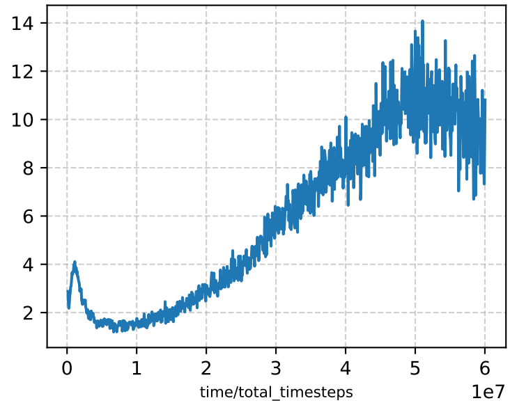
train/loss
