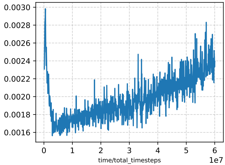
train/loss
