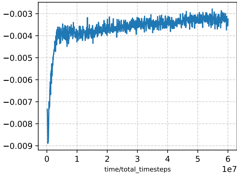
train/entropy_loss
