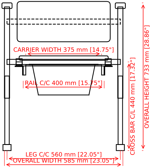
FRONT VIEW (slides on side rails, section through pan)
