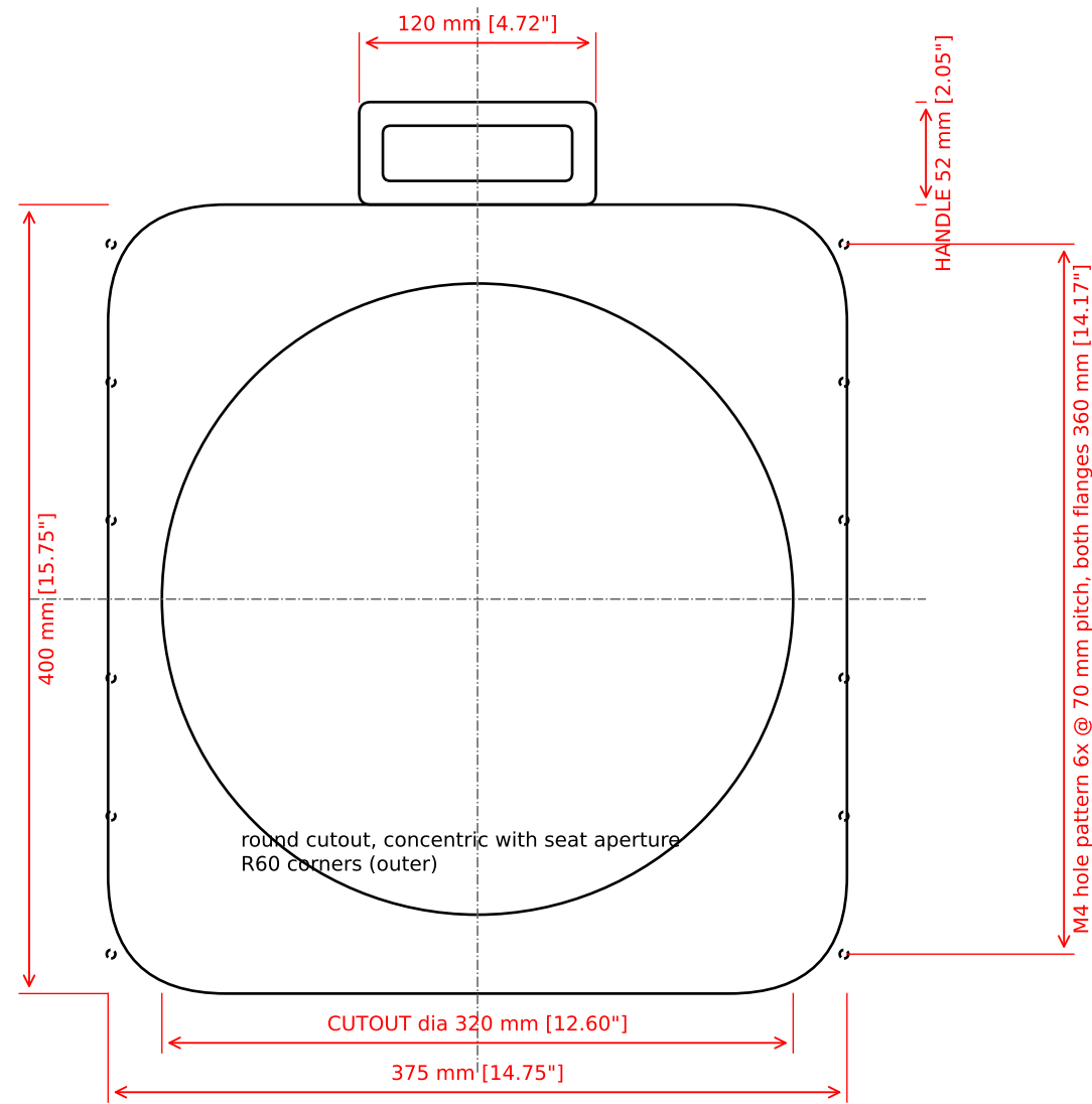
TOP VIEW (+Y = rear / pull direction, up on page)
