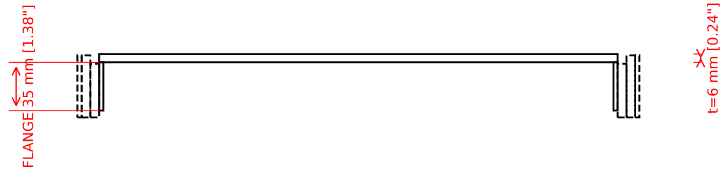
SECTION A-A (through X=0, looking from rear) - side flanges bolt to slide drawer members
