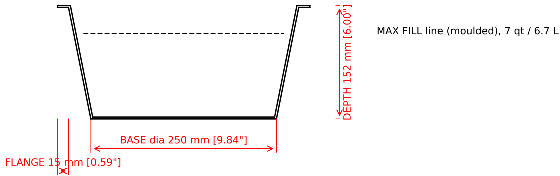
SECTION B-B (through centre)
