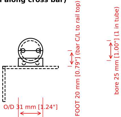
CLAMP BRACKET - END VIEW (2-piece saddle + foot, 30 mm long, seen along cross bar)
