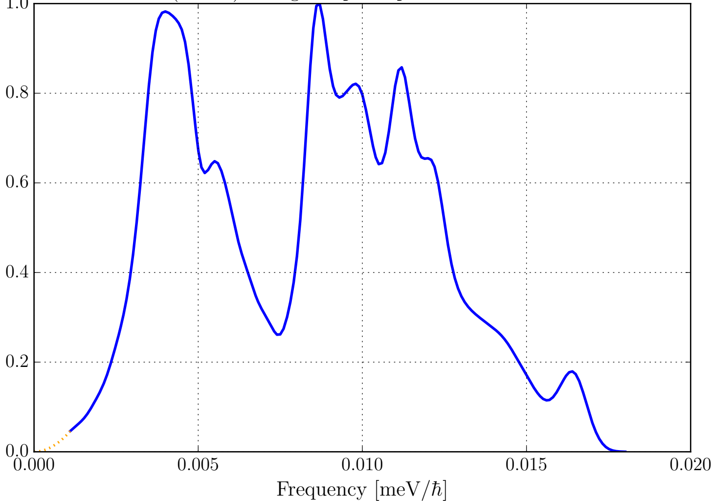
Phonon DOS (VDOS) for Ag in AgBr_sg225_SilverBromide.ncmat
