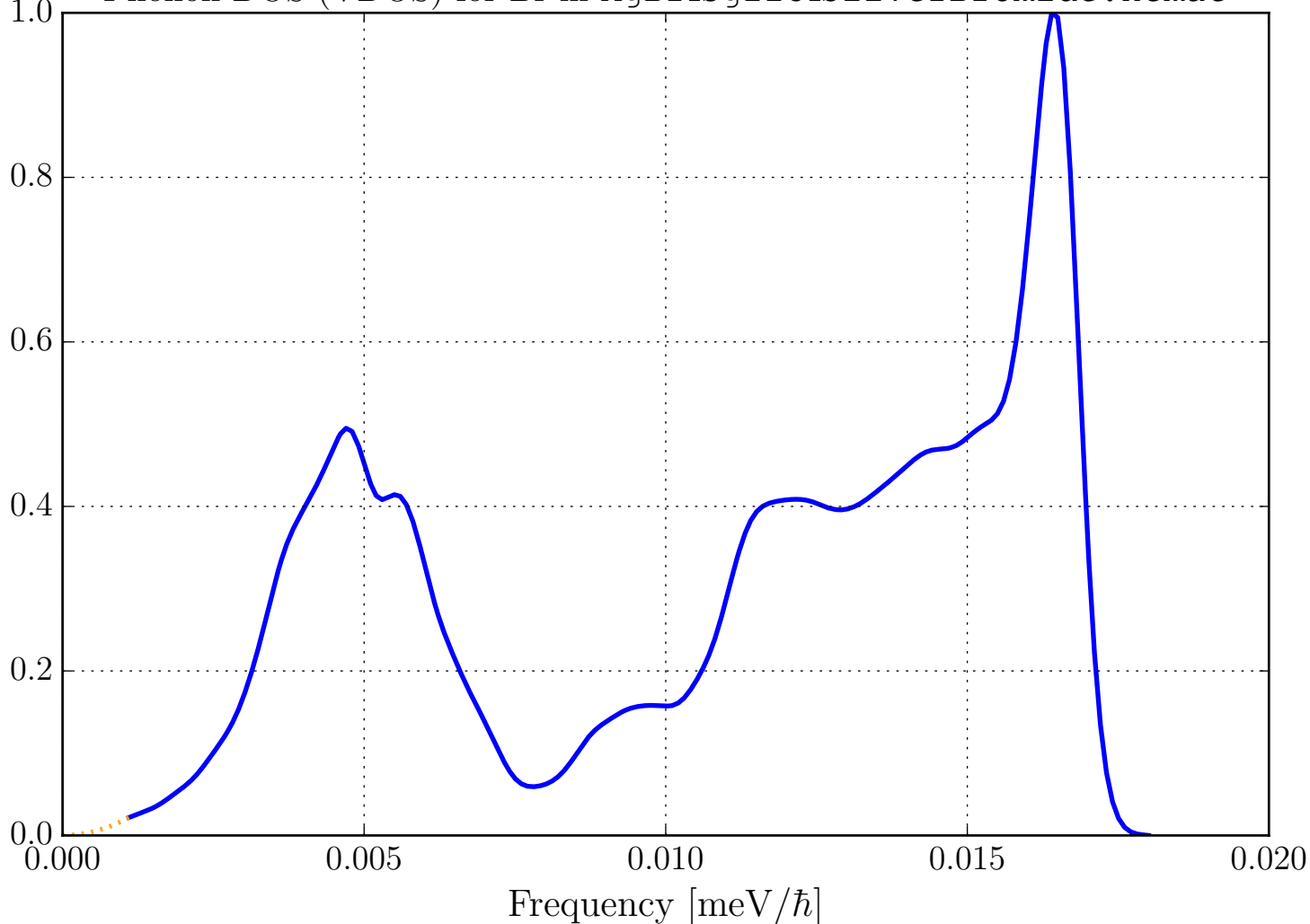
Phonon DOS (VDOS) for Br in AgBr_sg225_SilverBromide.ncmat
