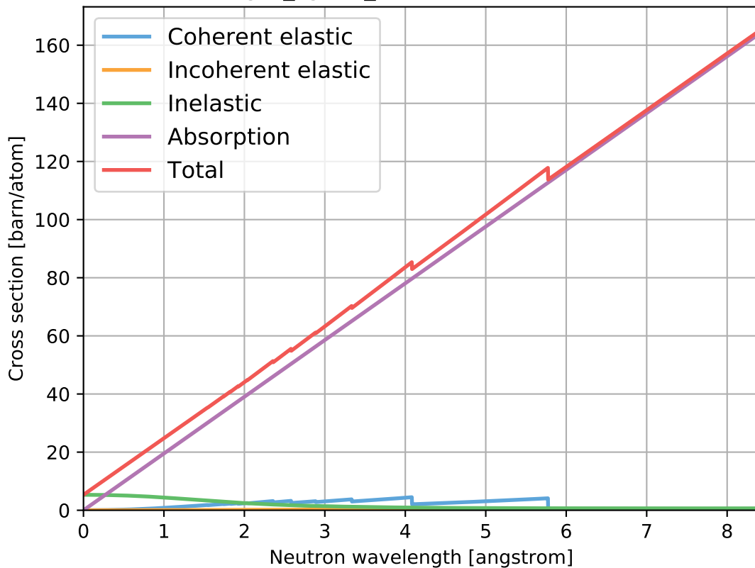
AgBr_sg225_SilverBromide.ncmat
