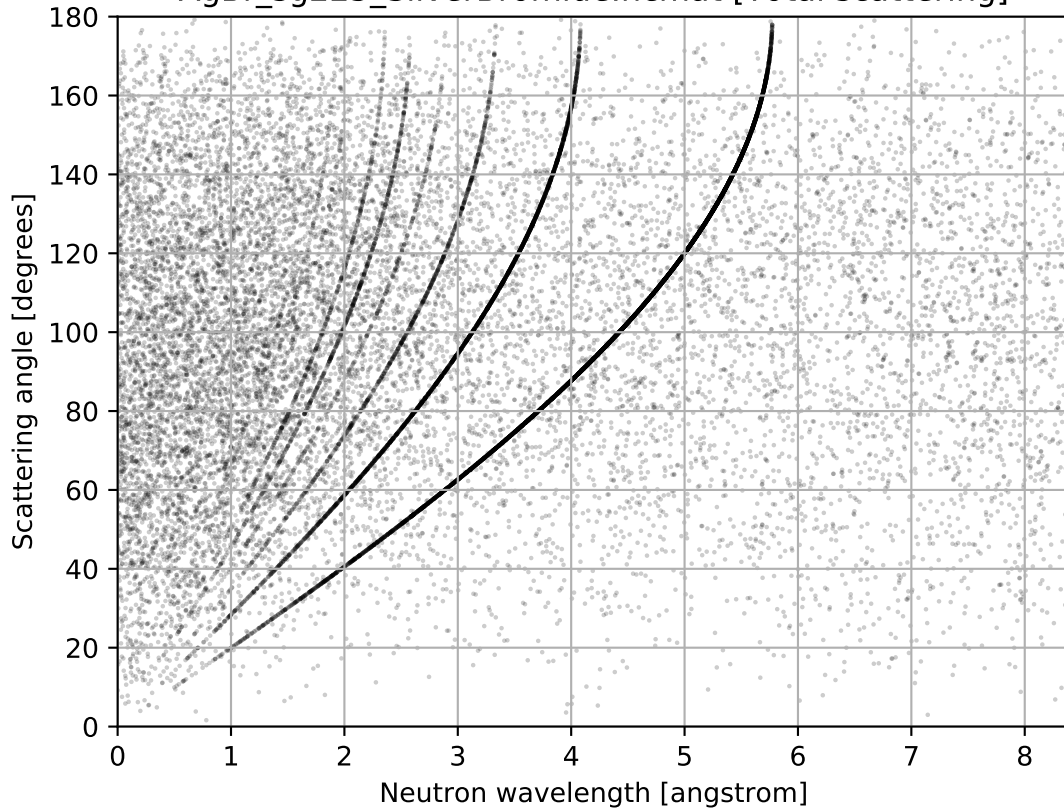
AgBr_sg225_SilverBromide.ncmat [Total scattering]
