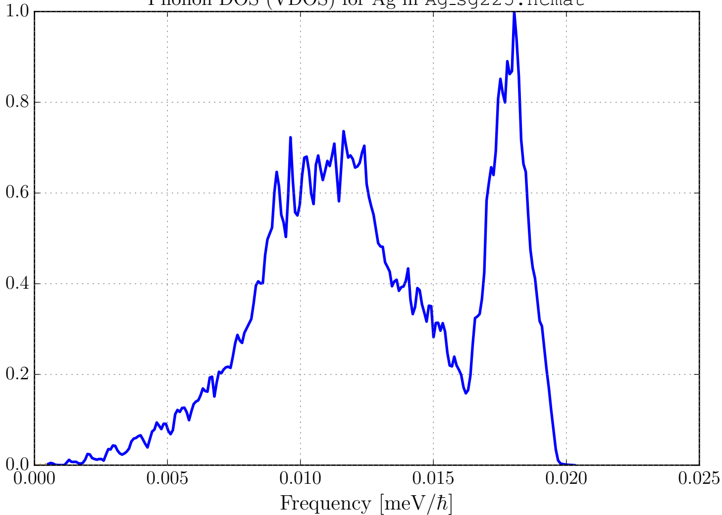
Phonon DOS (VDOS) for Ag in Ag_sg225.ncmat
