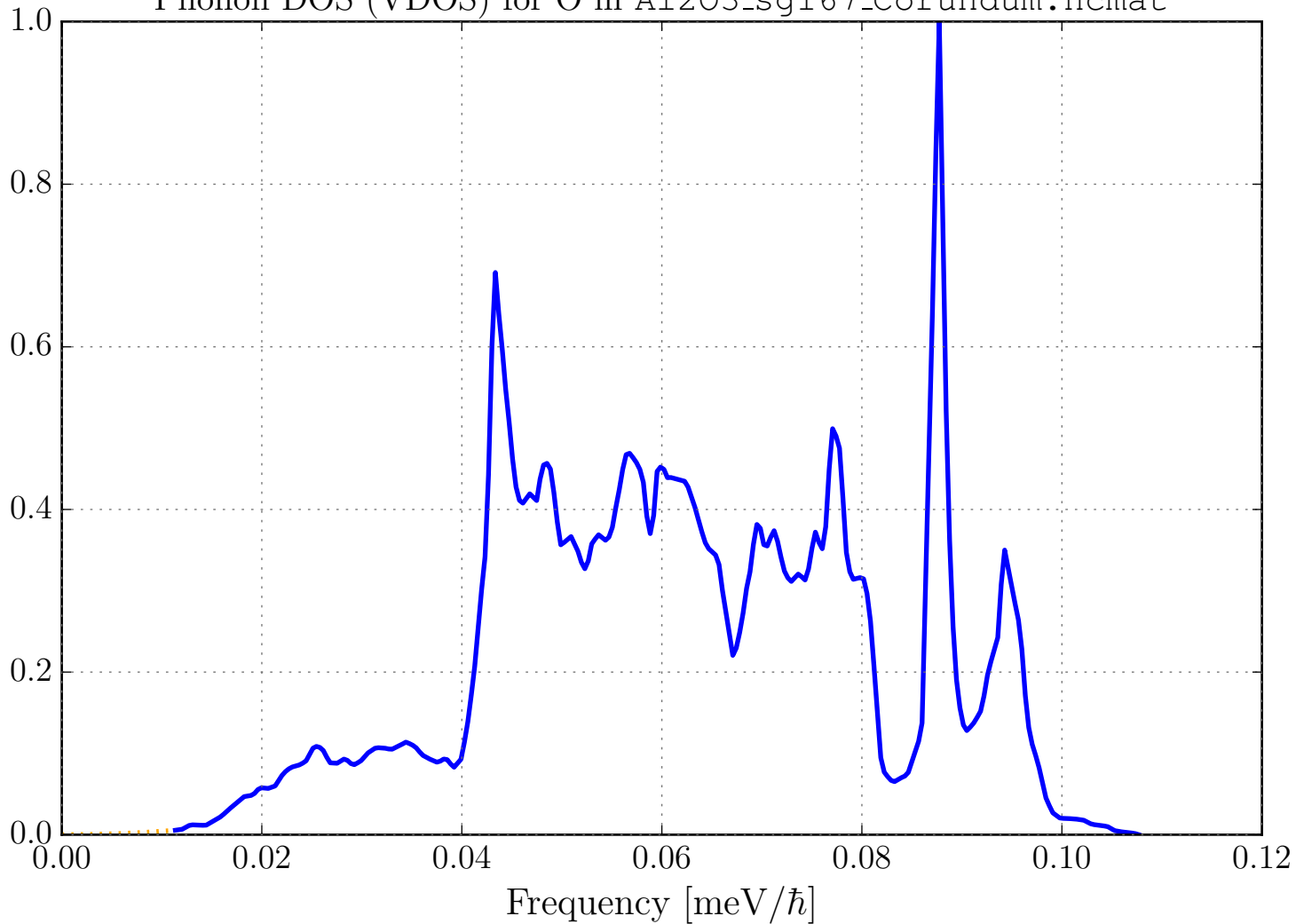
Phonon DOS (VDOS) for O in Al 2 O 3 _sg167_Corundum.ncmat
