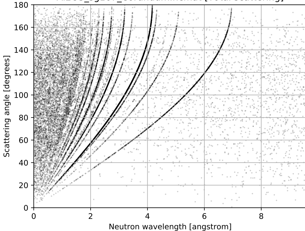
Al2O3_sg167_Corundum.ncmat [Total scattering]
