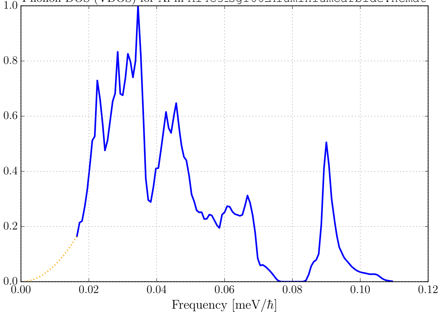
Phonon DOS (VDOS) for Al in Al4C3_sg166_AluminiumCarbide.ncmat
