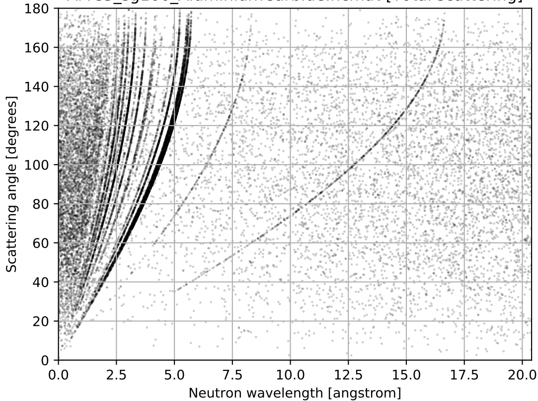
Al4C3_sg166_AluminiumCarbide.ncmat [Total scattering]
