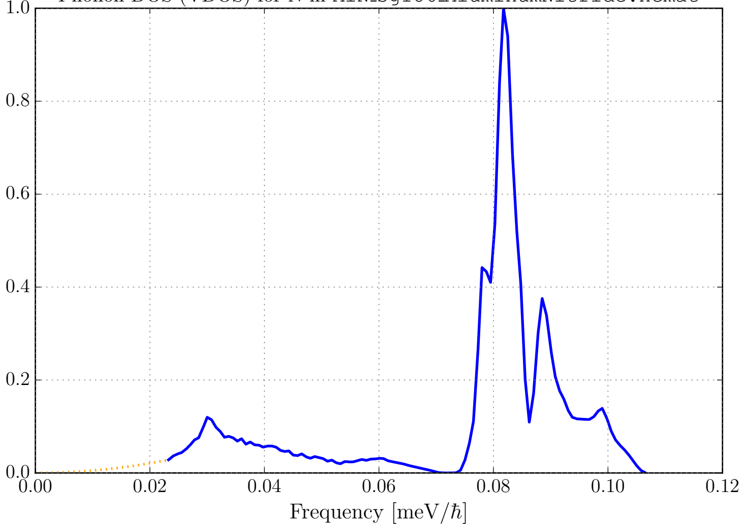
Phonon DOS (VDOS) for N in AlN_sg186_AluminumNitride.ncmat
