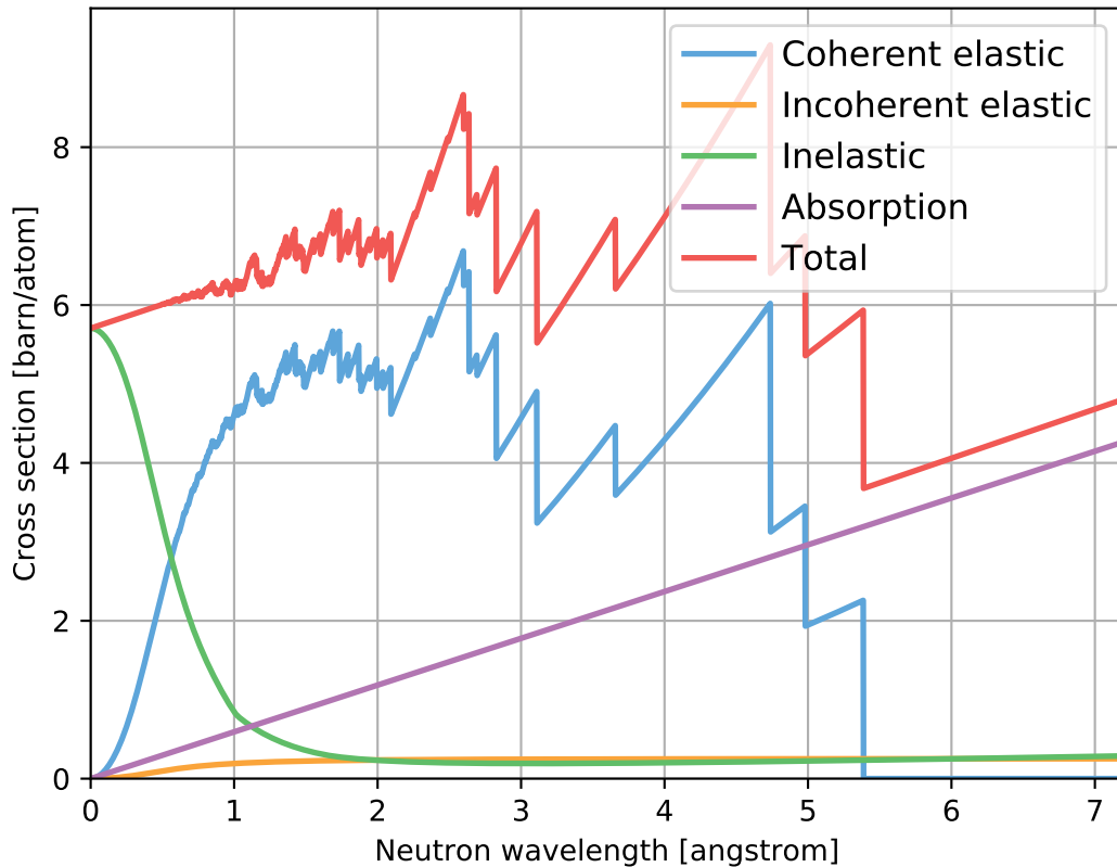
AlN_sg186_AluminumNitride.ncmat
