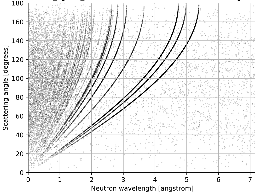
AlN_sg186_AluminumNitride.ncmat [Total scattering]
