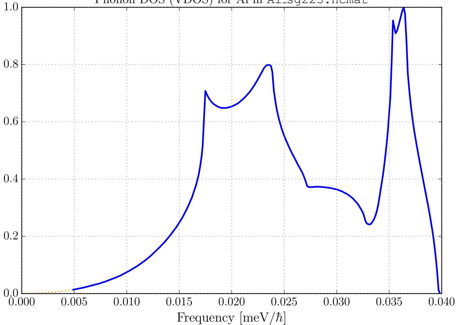
Phonon DOS (VDOS) for Al in Al_sg225.ncmat
