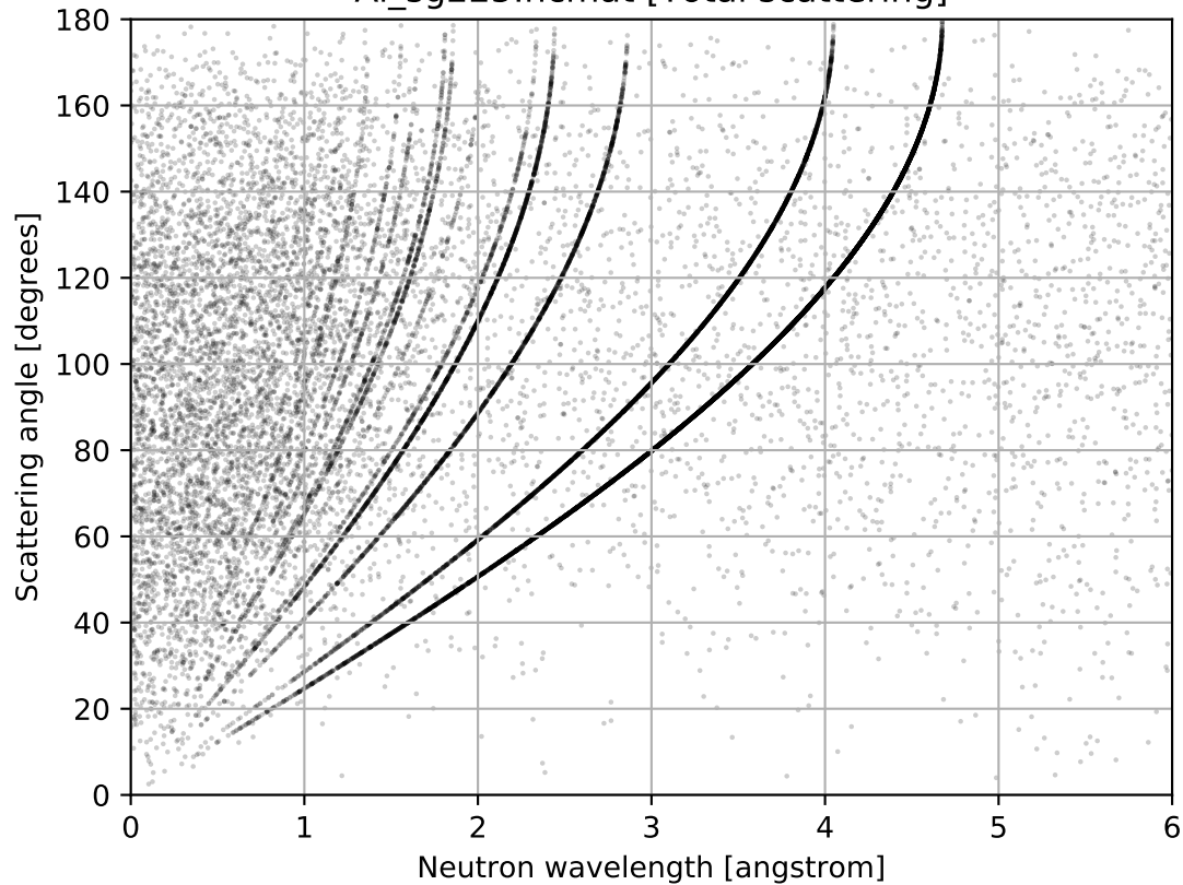
Al_sg225.ncmat [Total scattering]
