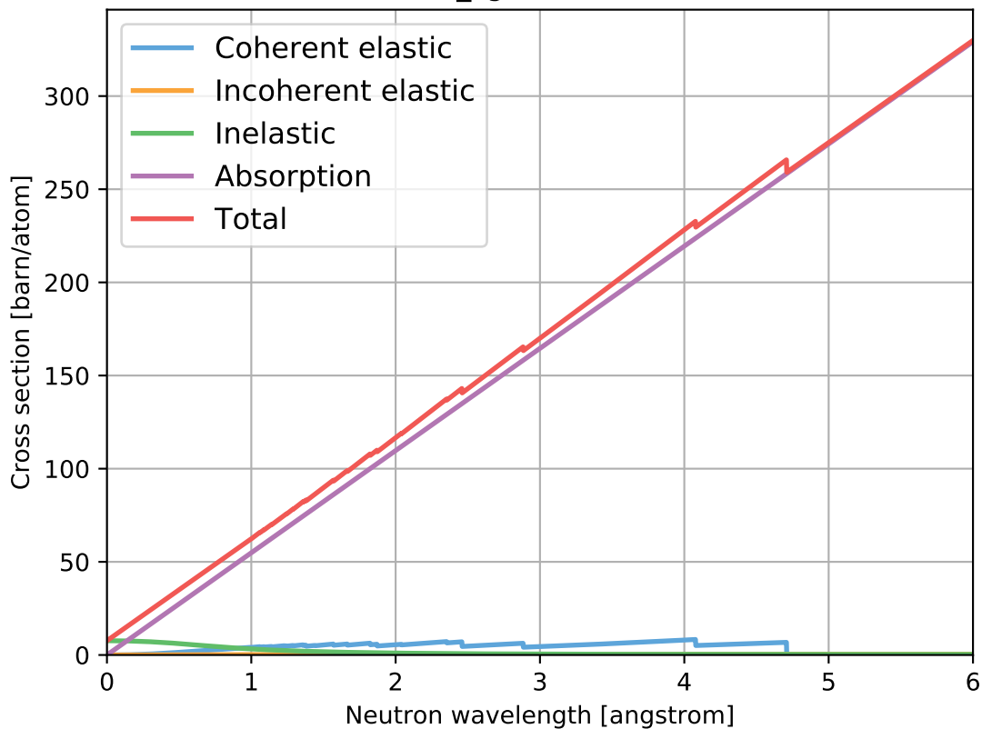
Au_sg225.ncmat
