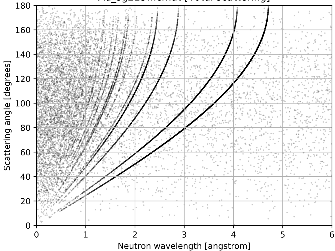
Au_sg225.ncmat [Total scattering]
