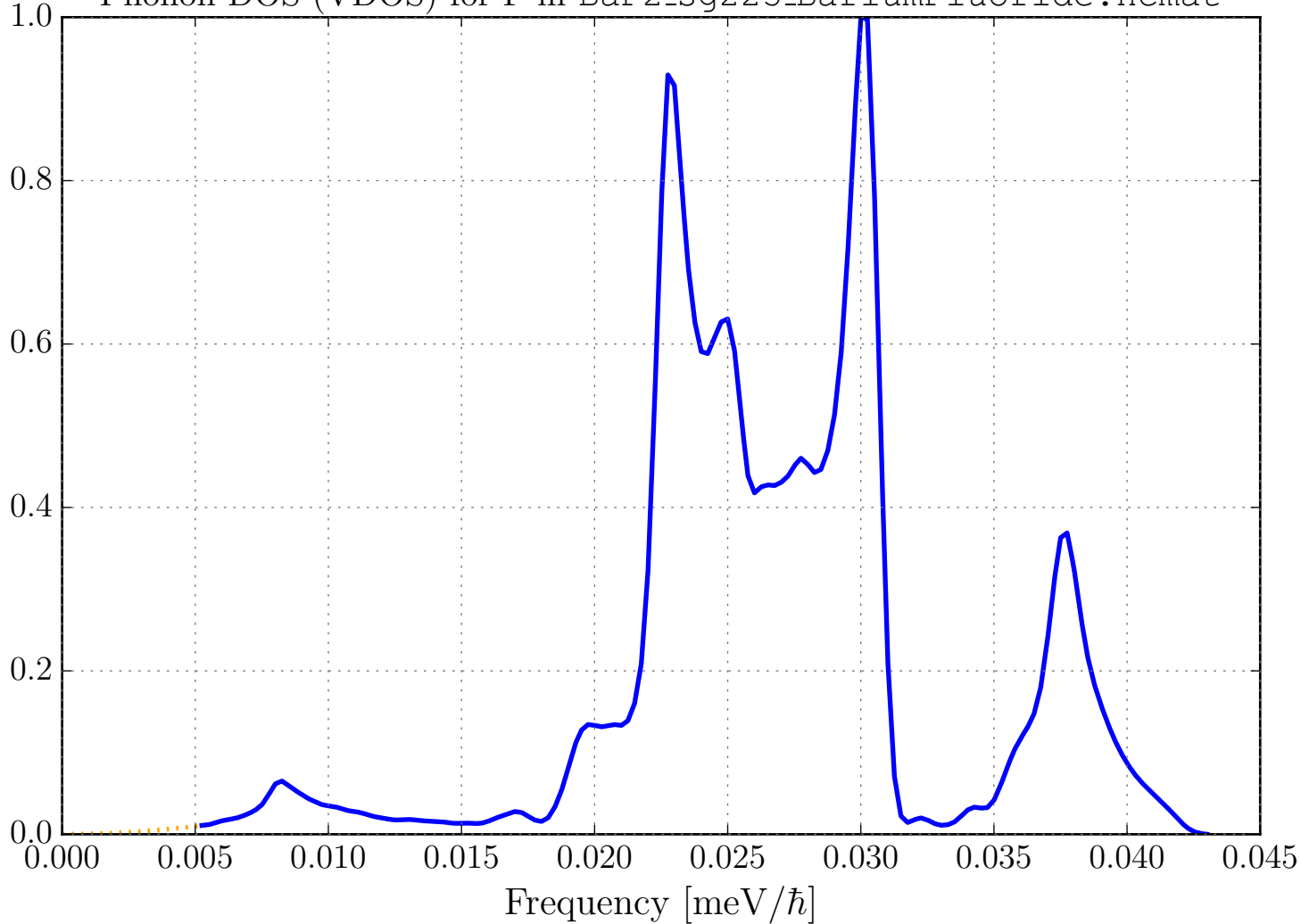
Phonon DOS (VDOS) for F in BaF2_sg225_BariumFluoride.ncmat
