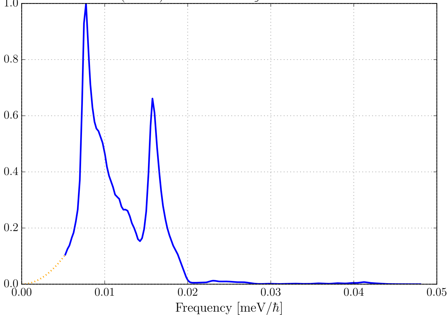
Phonon DOS (VDOS) for Ba in BaO_sg225_BariumOxide.ncmat
