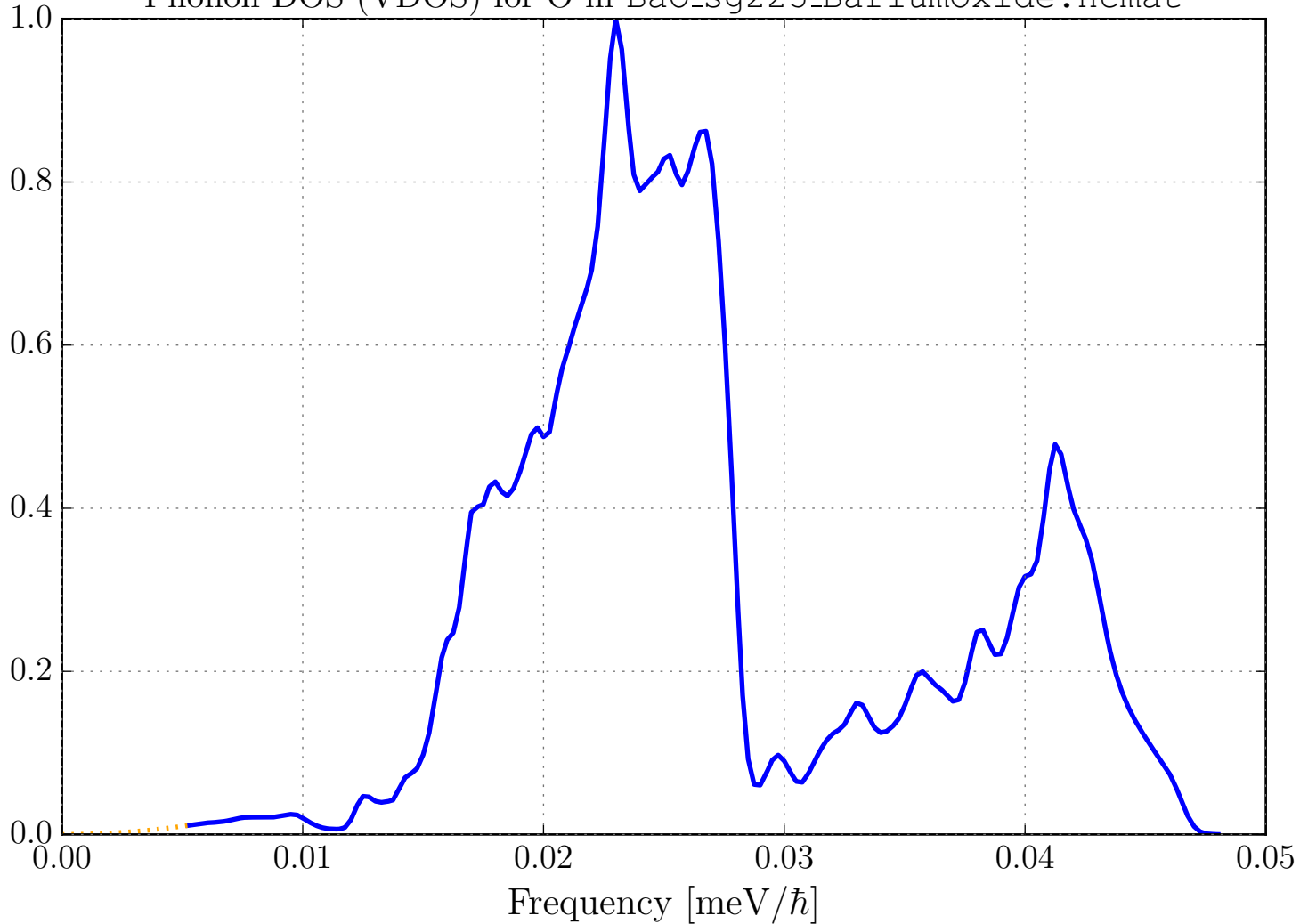
Phonon DOS (VDOS) for O in BaO_sg225_BariumOxide.ncmat
