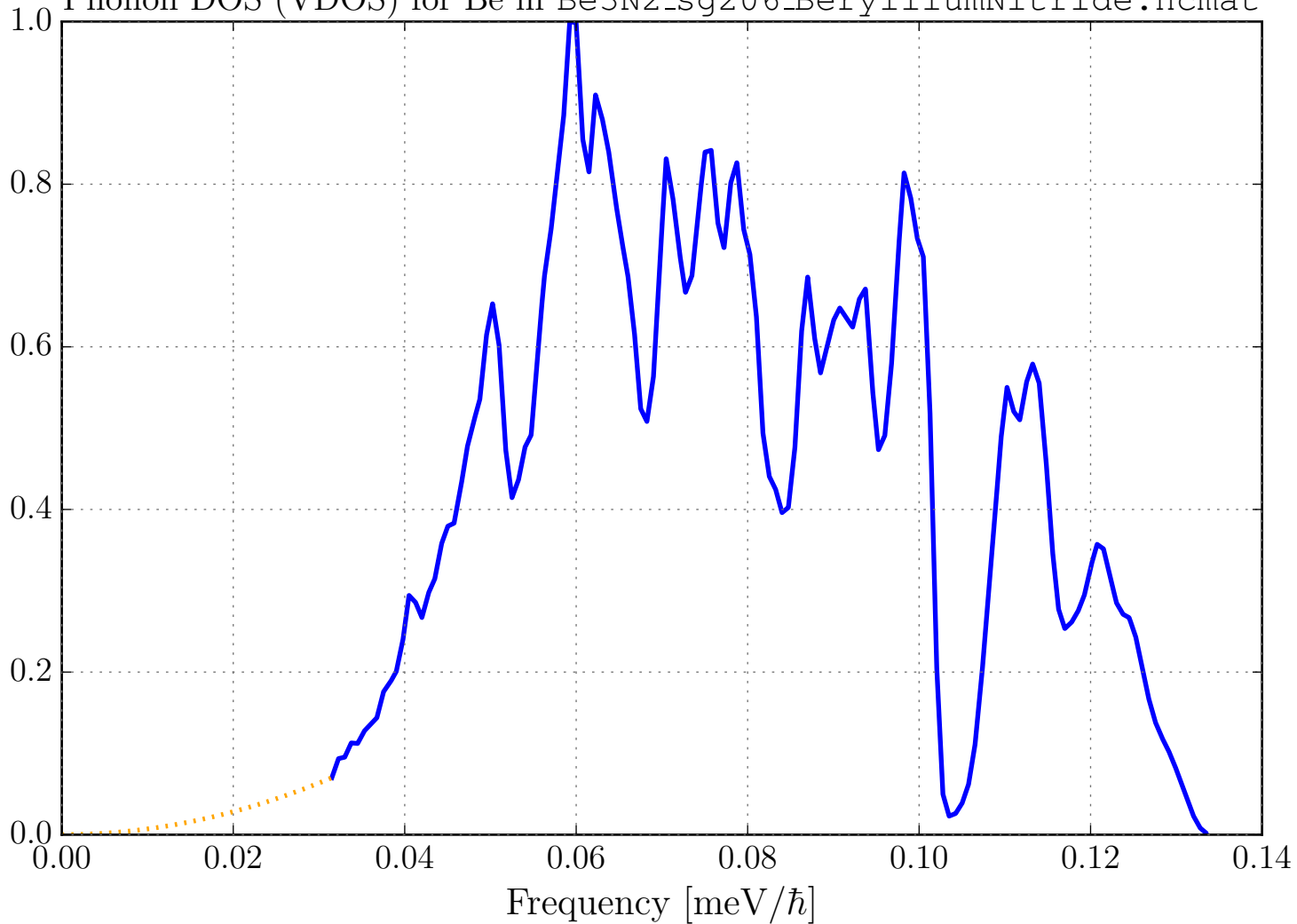
Phonon DOS (VDOS) for Be in Be3N2_sg206_BerylliumNitride.ncmat
