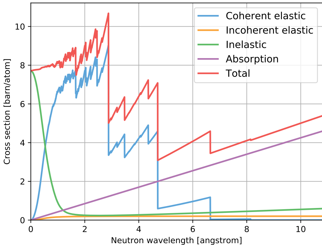
Be3N2_sg206_BerylliumNitride.ncmat
