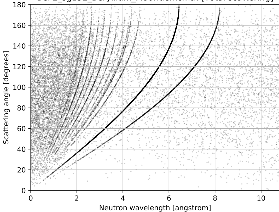
BeF2_sg152_Beryllium_Fluoride.ncmat [Total scattering]
