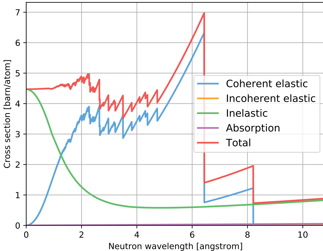
BeF2_sg152_Beryllium_Fluoride.ncmat
