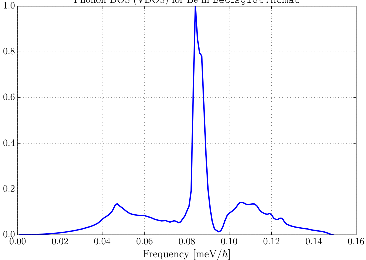
Phonon DOS (VDOS) for Be in BeO_sg186.ncmat
