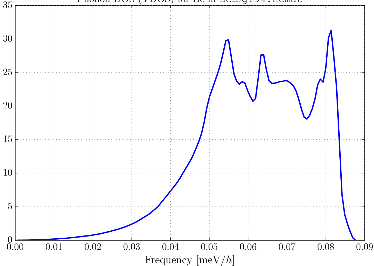
Phonon DOS (VDOS) for Be in Be_sg194.ncmat
