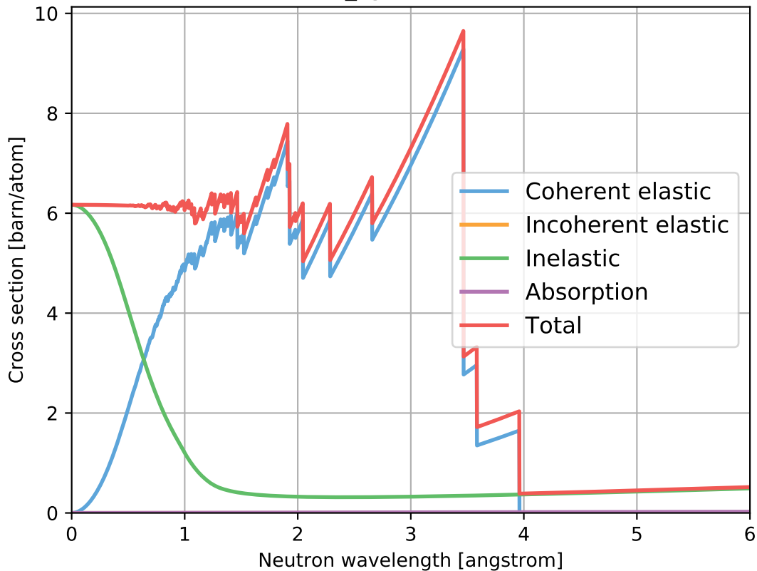
Be_sg194.ncmat
