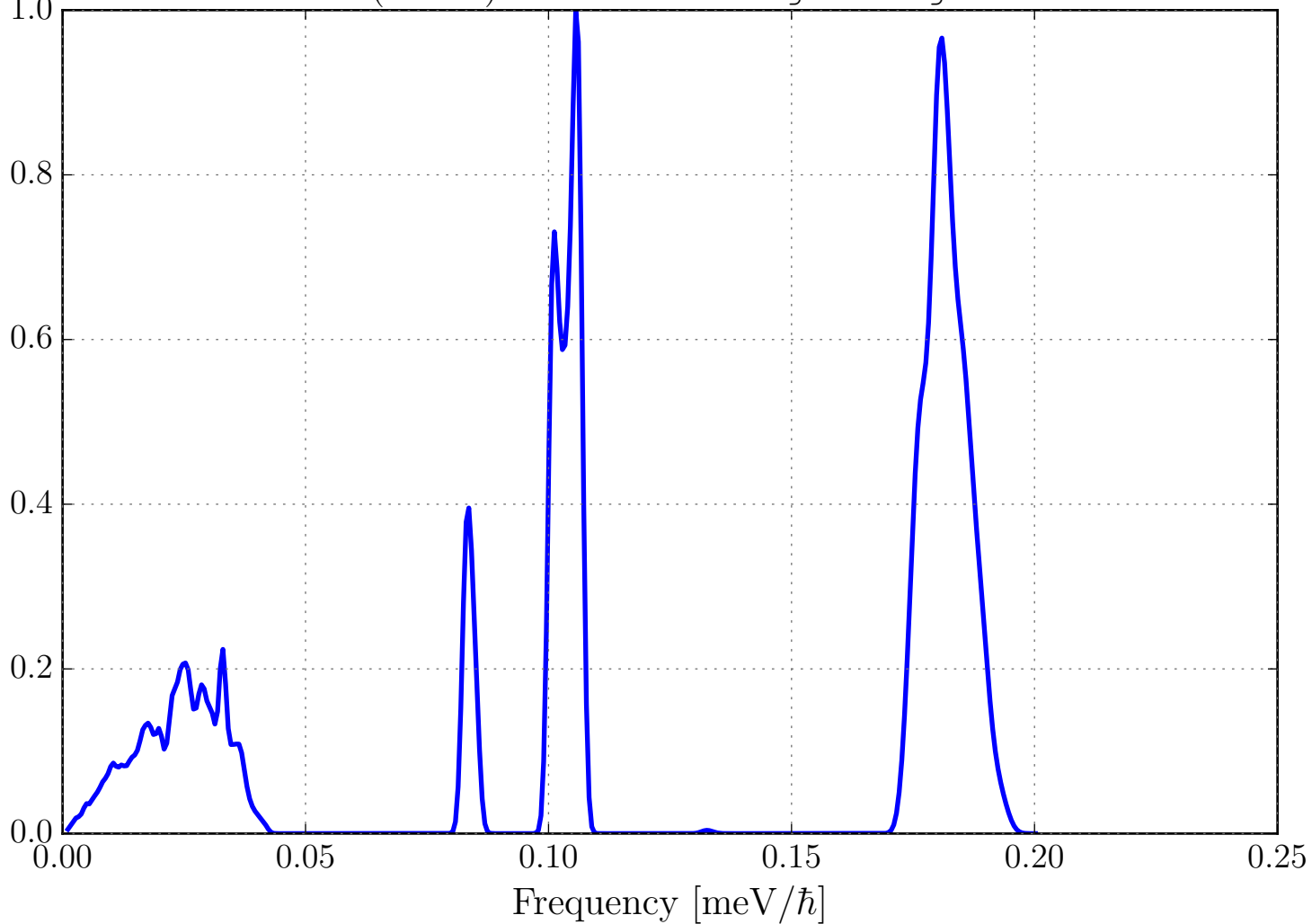
Phonon DOS (VDOS) for C in CaCO3_sg62_Aragonite.ncmat
