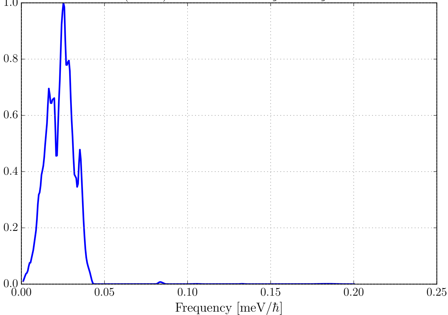
Phonon DOS (VDOS) for Ca in CaCO3_sg62_Aragonite.ncmat
