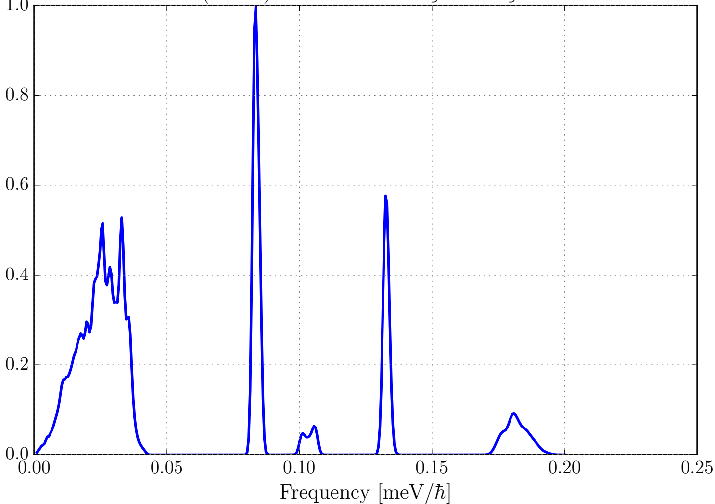
Phonon DOS (VDOS) for O in CaCO3_sg62_Aragonite.ncmat
