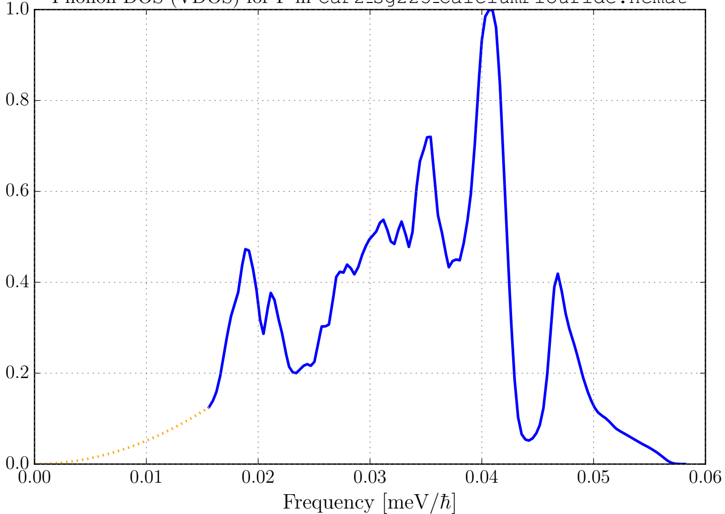
Phonon DOS (VDOS) for F in CaF2_sg225_CalciumFlouride.ncmat
