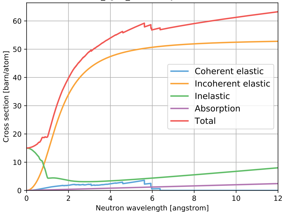
CaH2_sg62_CalciumHydride.ncmat
