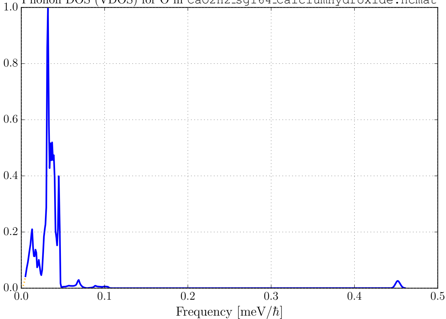
Phonon DOS (VDOS) for O in CaO2H2_sg164_CalciumHydroxide.ncmat
