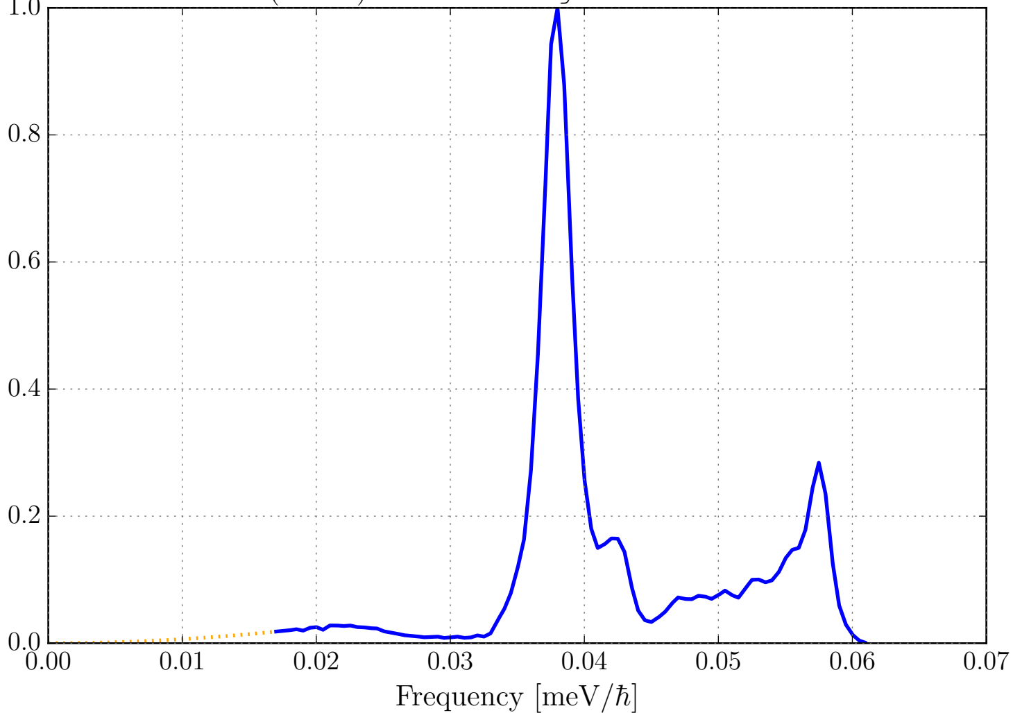
Phonon DOS (VDOS) for O in CaO_sg225_CalciumOxide.ncmat
