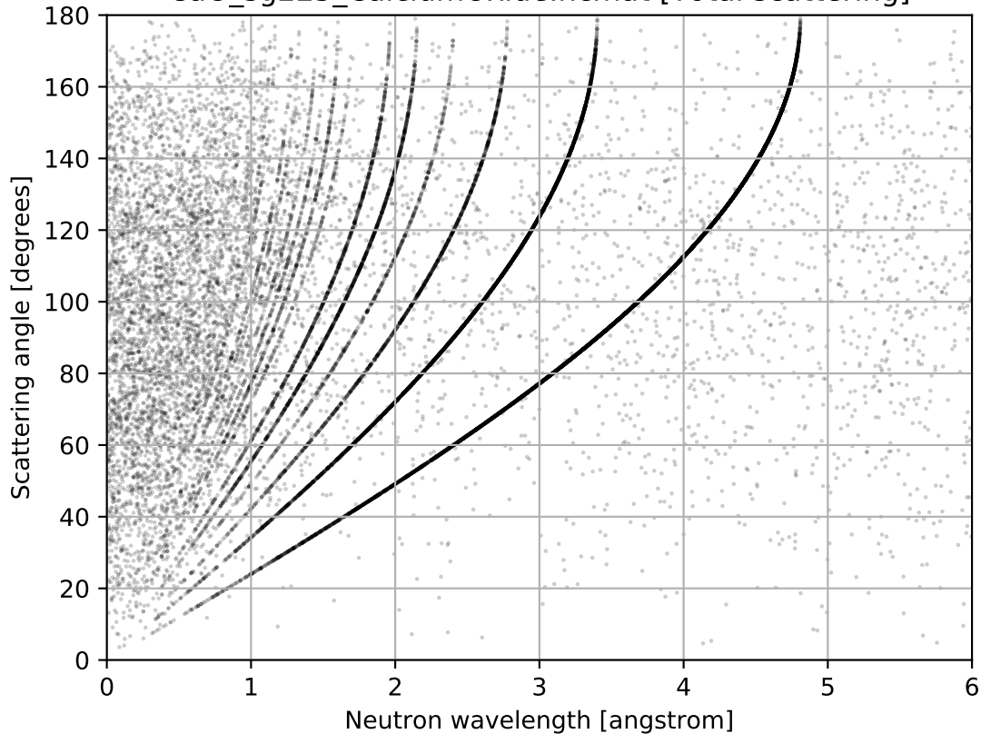
CaO_sg225_CalciumOxide.ncmat [Total scattering]
