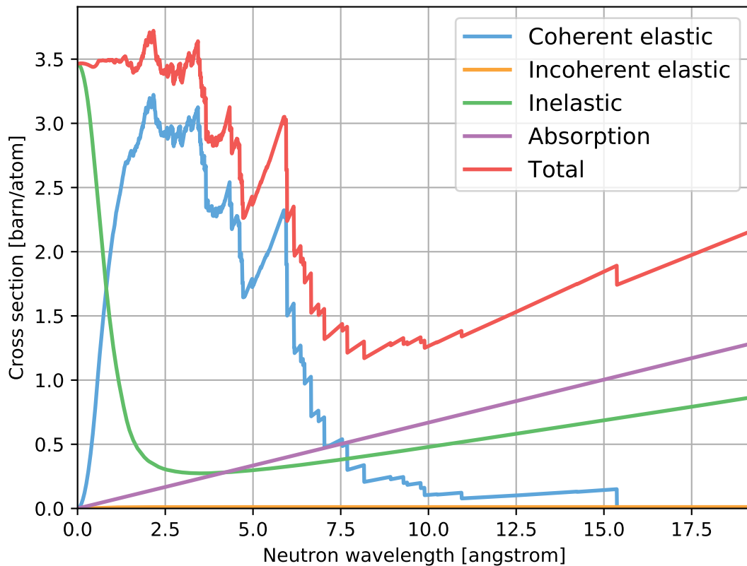
CaSiO3_sg2_Wollastonite.ncmat [dcutoff=0.3]
