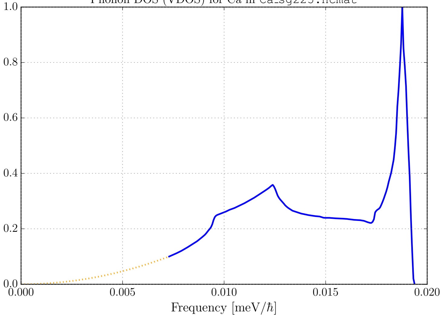
Phonon DOS (VDOS) for Ca in Ca_sg225.ncmat
