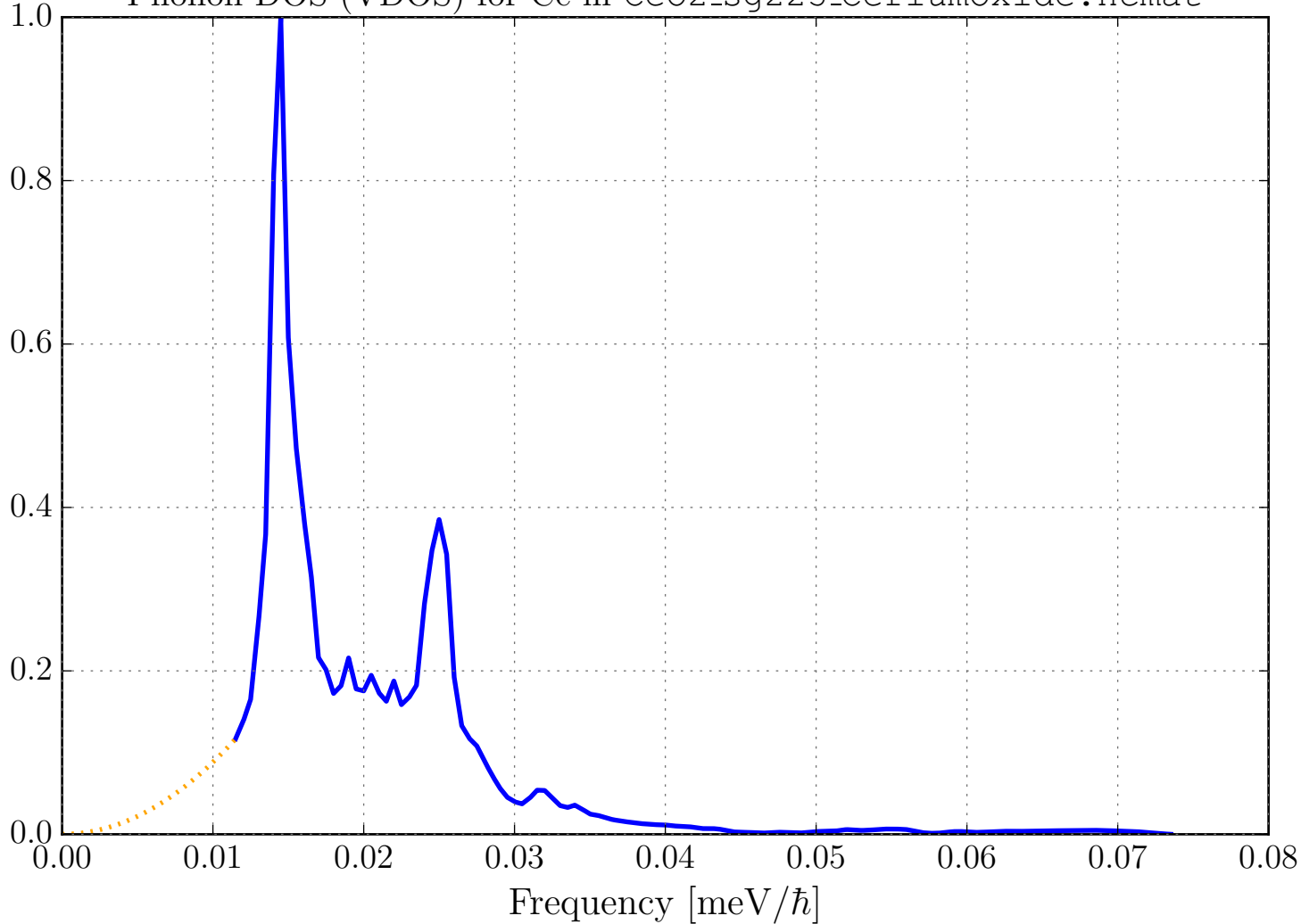
Phonon DOS (VDOS) for Ce in CeO2_sg225_CeriumOxide.ncmat
