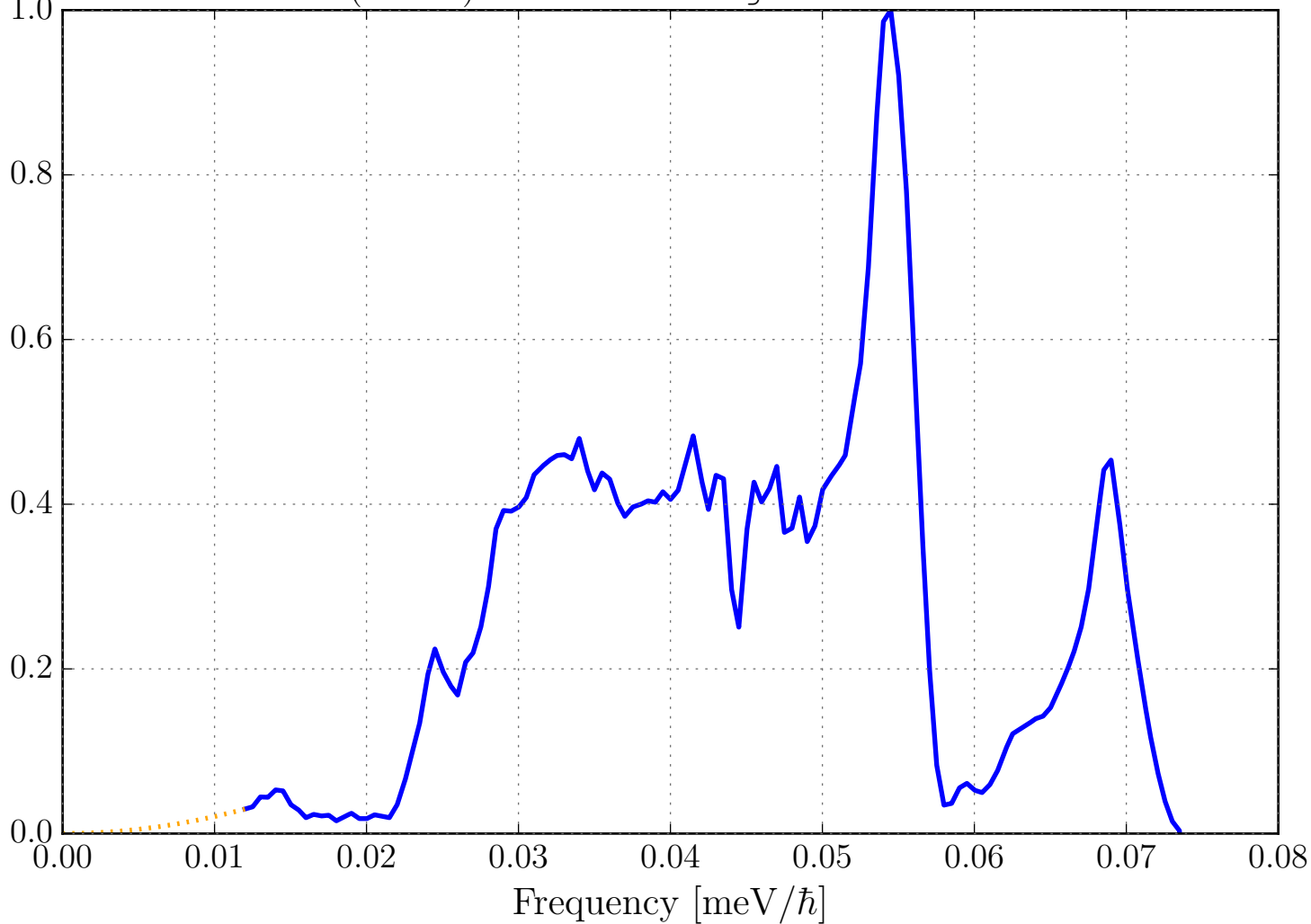
Phonon DOS (VDOS) for O in CeO 2 _sg225_CeriumOxide.ncmat
