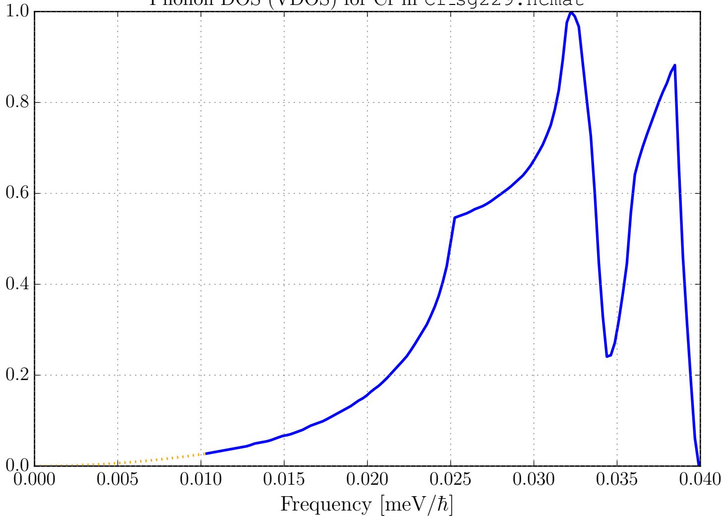
Phonon DOS (VDOS) for Cr in Cr_sg229.ncmat
